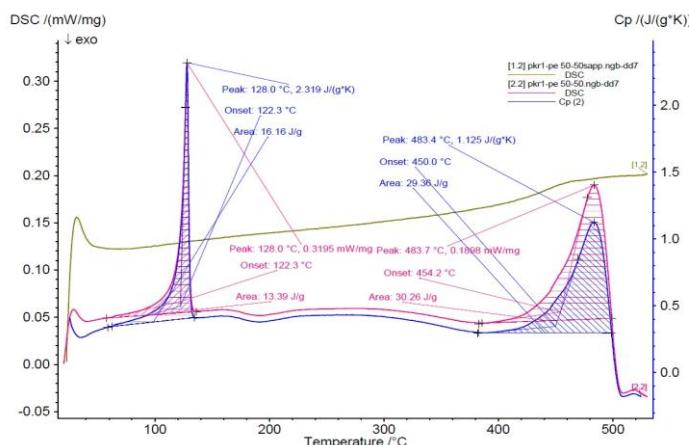
Figure 3. DSC thermogram of HDPE+PKR1 composite.
