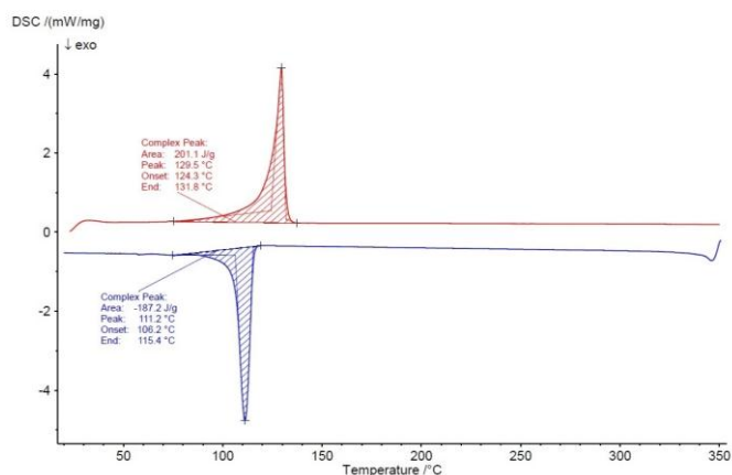
Figure 2. DSC thermogram of polyvinylidene fluoride (PVDF).
