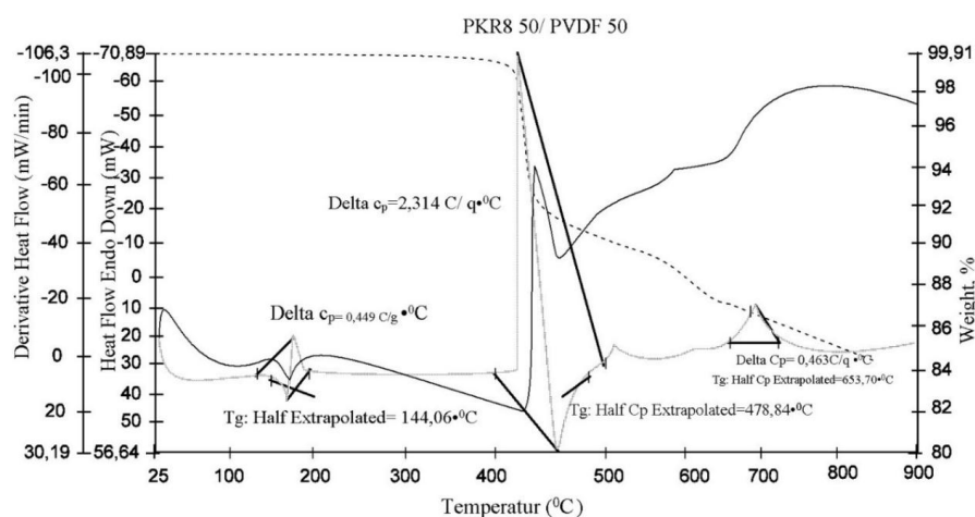
Figure 6. Thermogravimetric (TG) spectrum of PVDF+PCR8 composite.
