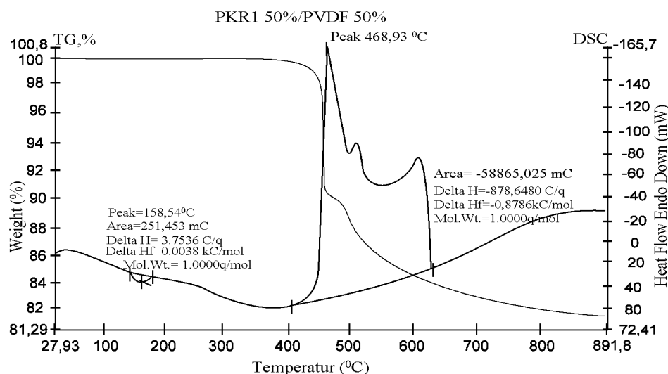
Figure 5. Thermogravimetric (TG) spectrum of PVDF+PKR1composite.
