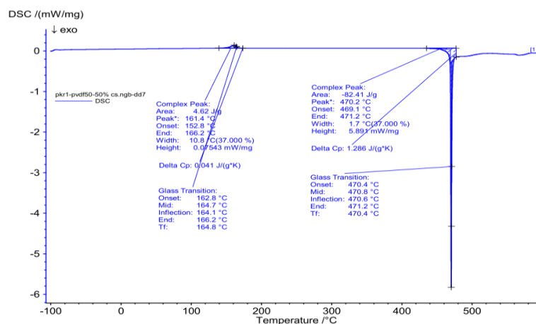
Figure 4. DSC thermogram of PVDF+PCR1 composite.
