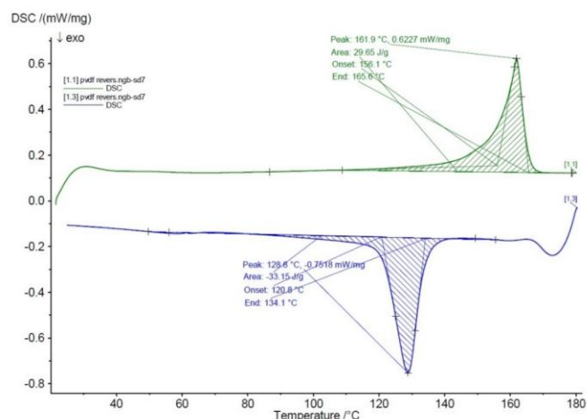
Figure 1. DSC thermogram of high-density polyethylene (HDPE)
